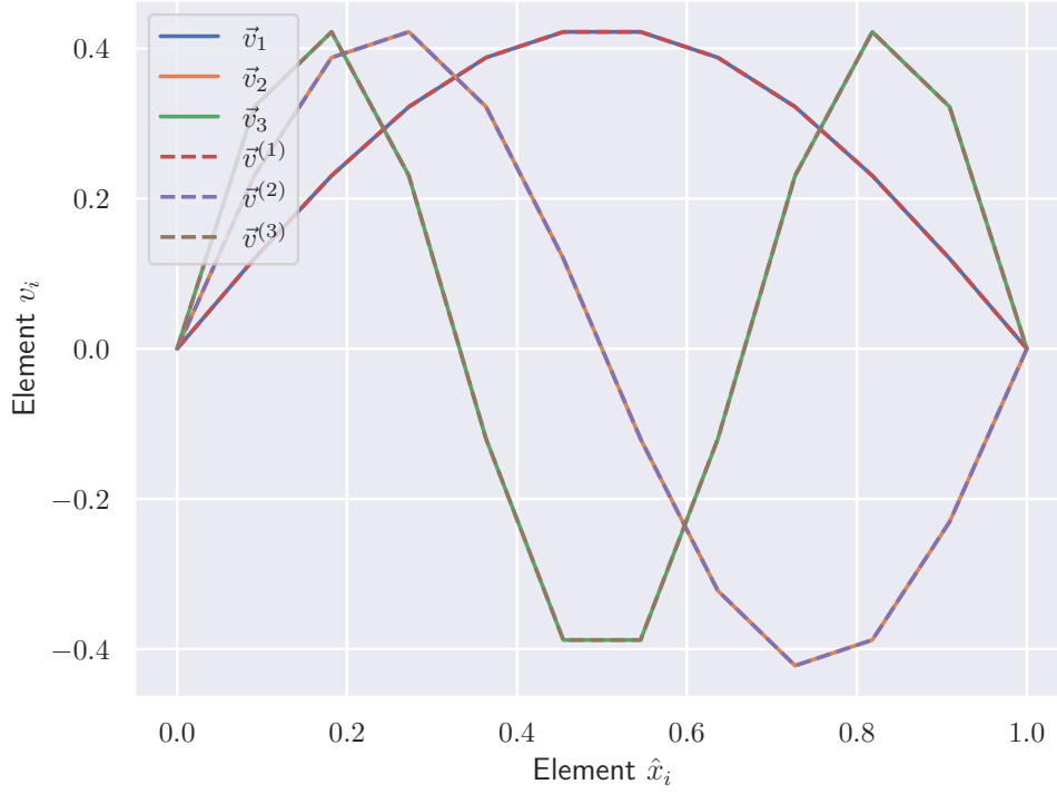
FIG. 2. The plot is showing the elements of eigenvector \vec{v}_1, \vec{v}_2, \vec{v}_3 , corresponding to the three lowest eigenvalues of matrix \mathbf{A}(10 \times 10) , against the position \hat{x} . The analytical eigenvectors \vec{v}^{(1)}, \vec{v}^{(2)}, \vec{v}^{(3)} are also included in the plot.
