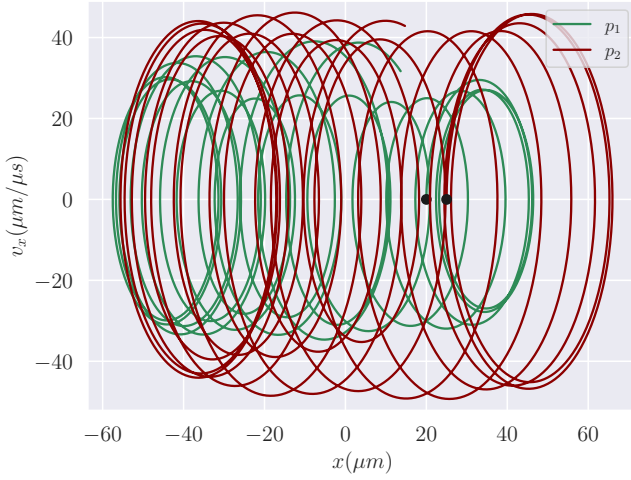
FIG. 8. Particle trajectory at a given position x , with particle interaction. The black dot marks the starting position of each particle.
