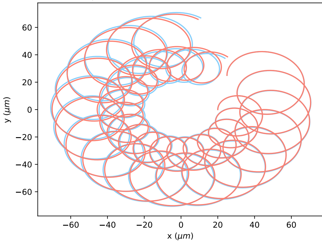
2 particles with and without interactions.
