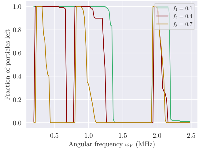
FIG. 11. Exploring particles
