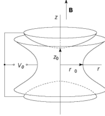
FIG. 1. The basic configuration of a hyperbolic Penning trap [? ]. Electric potential V_0 is applied to the electrodes in end caps (top and bottom), and in the ring (middle). The magnetic field is denoted as \mathbf{B} , the distance from the center to the end caps are denoted as z_0 , and the radial distance as r_0 .
