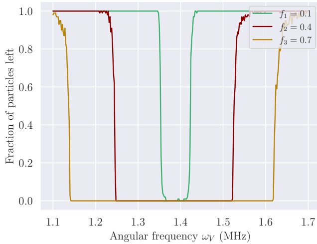
FIG. 12. Exploring different angular frequencies more closely
